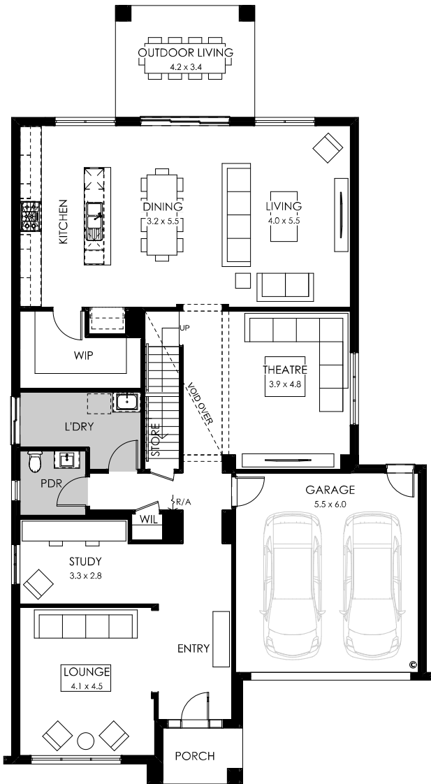
GROUND FLOOR
