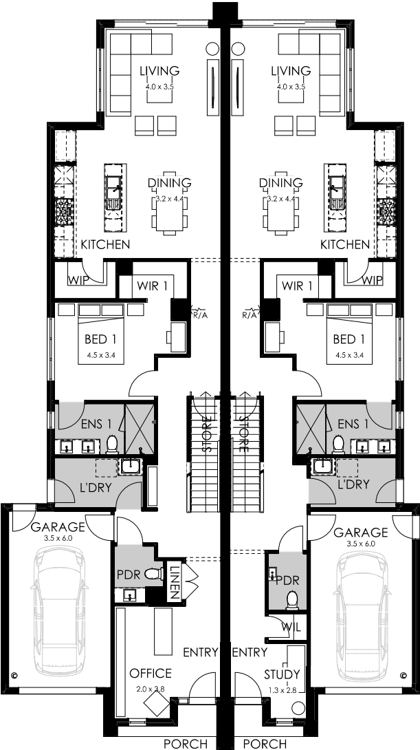
Spencer 28 Ground floor
