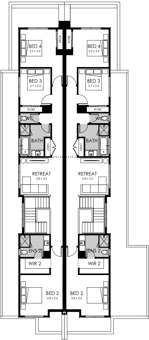
Franklin 28 First floor
