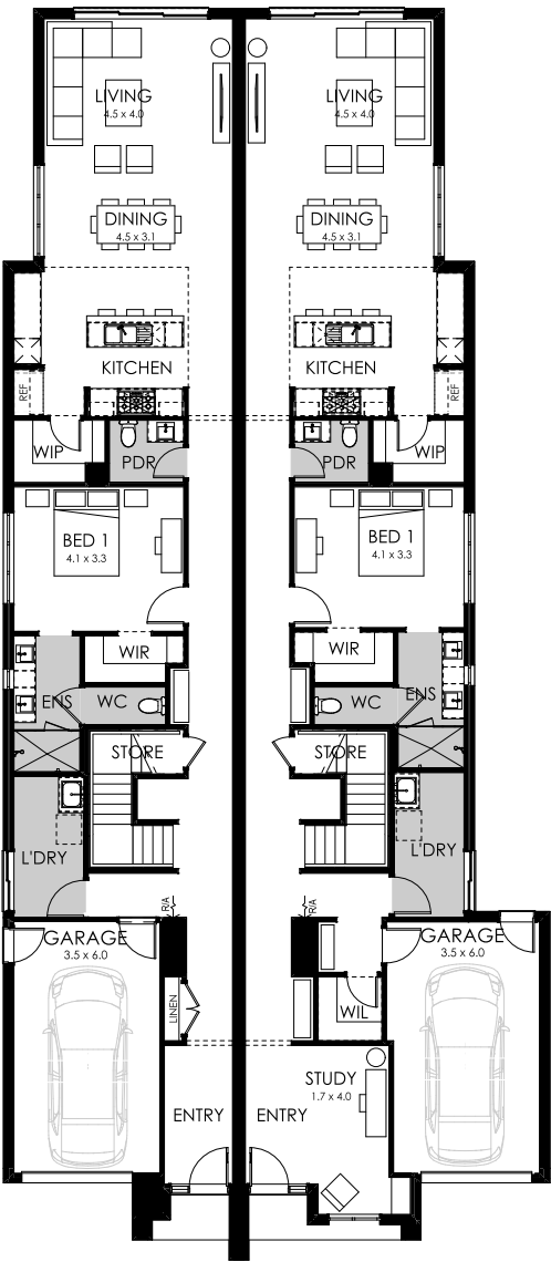
Franklin 28 Ground floor
